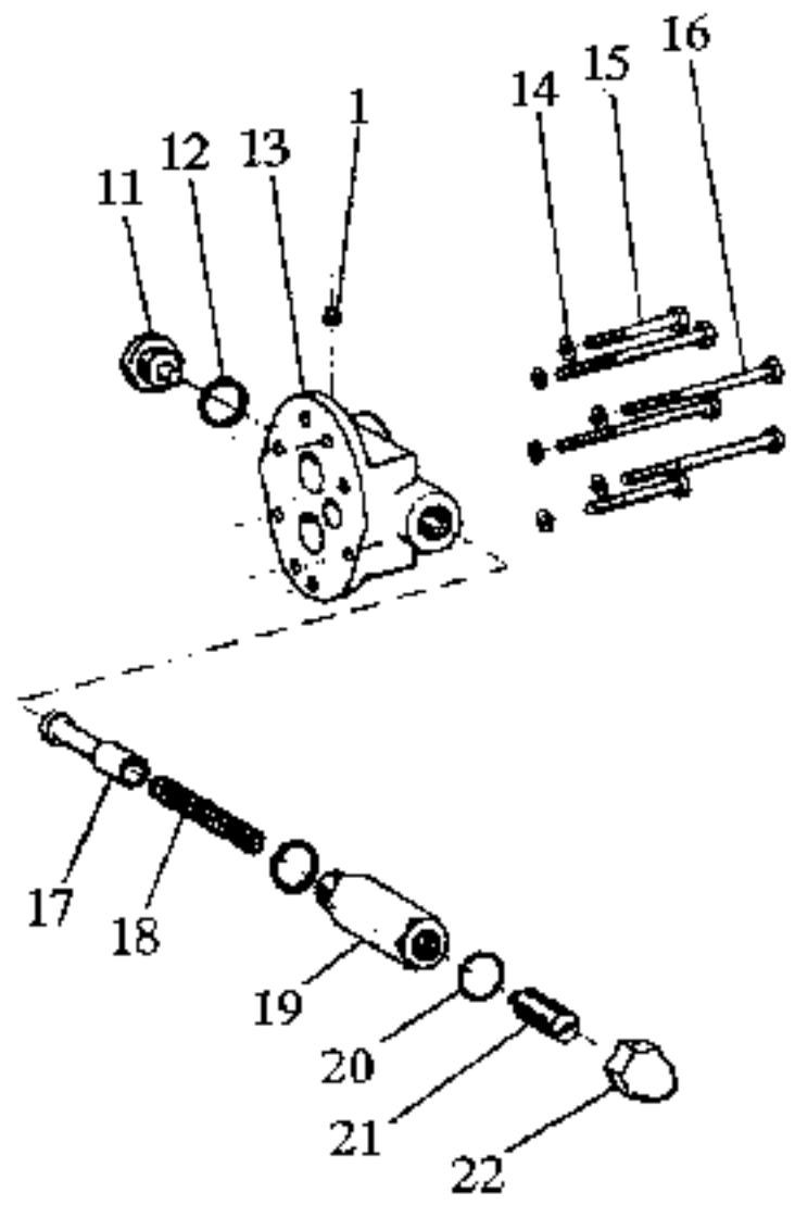
RIGHT HAND PUMP
